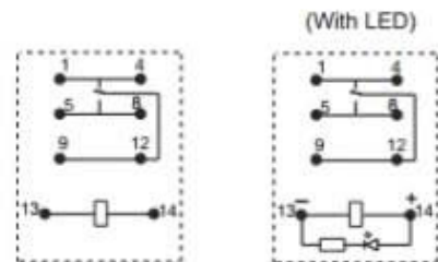
Wiring Diagram
