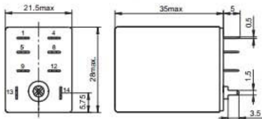
Outline Dimensions
