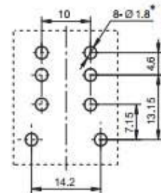
Mounting holes
