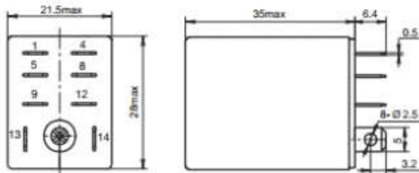
Outline Dimensions
